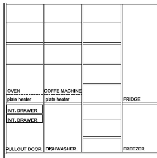
TALL UNITS - Internal arrangement
